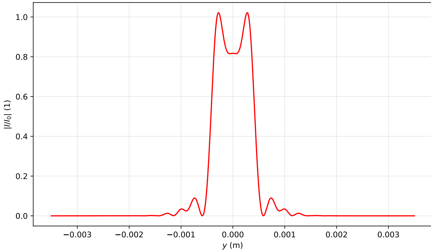
Intensity profile I(x=0, y, z=1.194)/I_0 , \text{Pin}=3.0\text{Pcr} , artificial time
